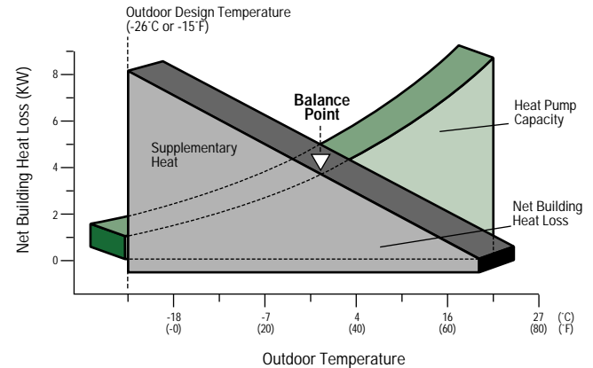
Figure 16: Balance Point for a Typical Air-Source Heat Pump
